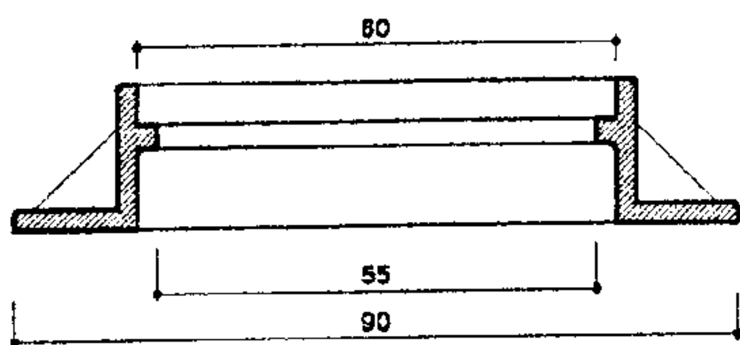
FRAME SECTION
