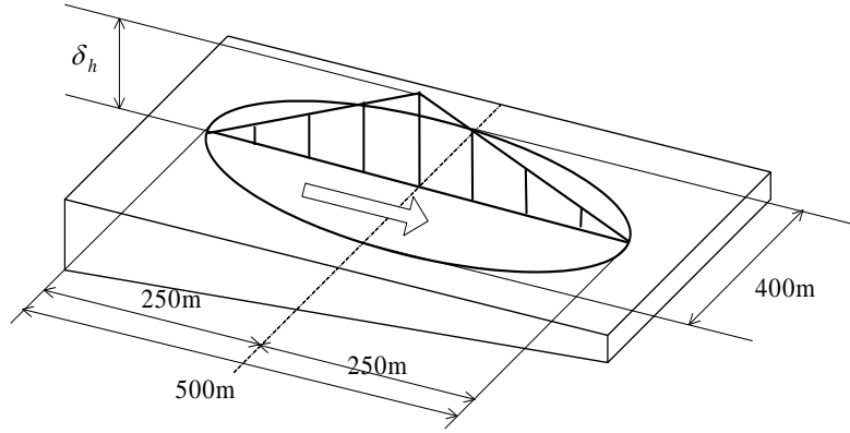
Fig. 4-2 distribution of ground horizontal displacement at steep ground
