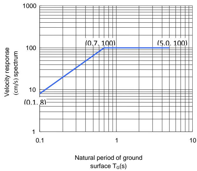
Fig. 3-4 velocity response spectrum for the risk level 2
