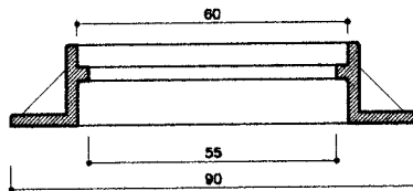
FRAME SECTION
