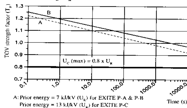
TOV capability for surge arrester type EXLIM P expressed in multiples of U_R ( T_R )
