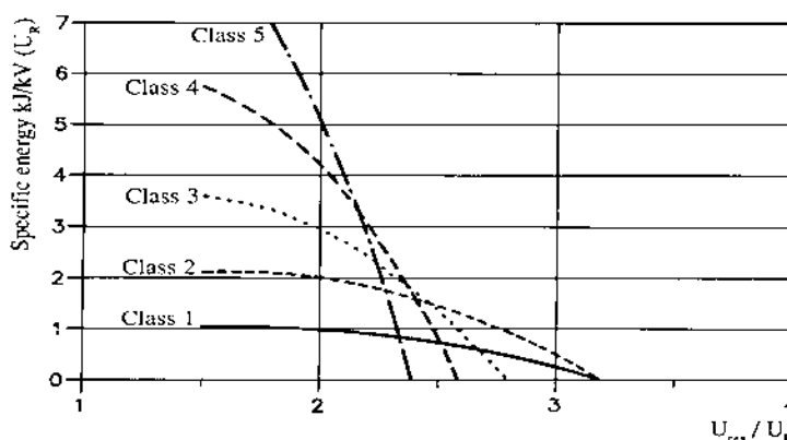
Absorbed specific energy kJ/kV for IEC line discharge classes
