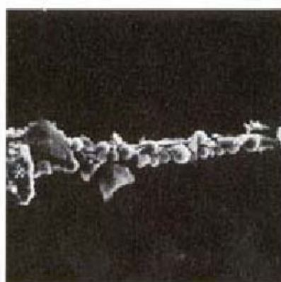
Fig. 1.3.16 S.E.M. 1000X | 20 μm |
