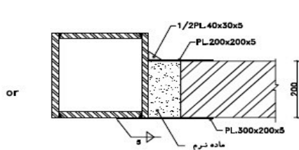
SEC. 2-2 S.C.: 1/10
